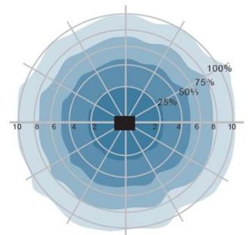
Ceiling mounting pattern (Unit: m)
